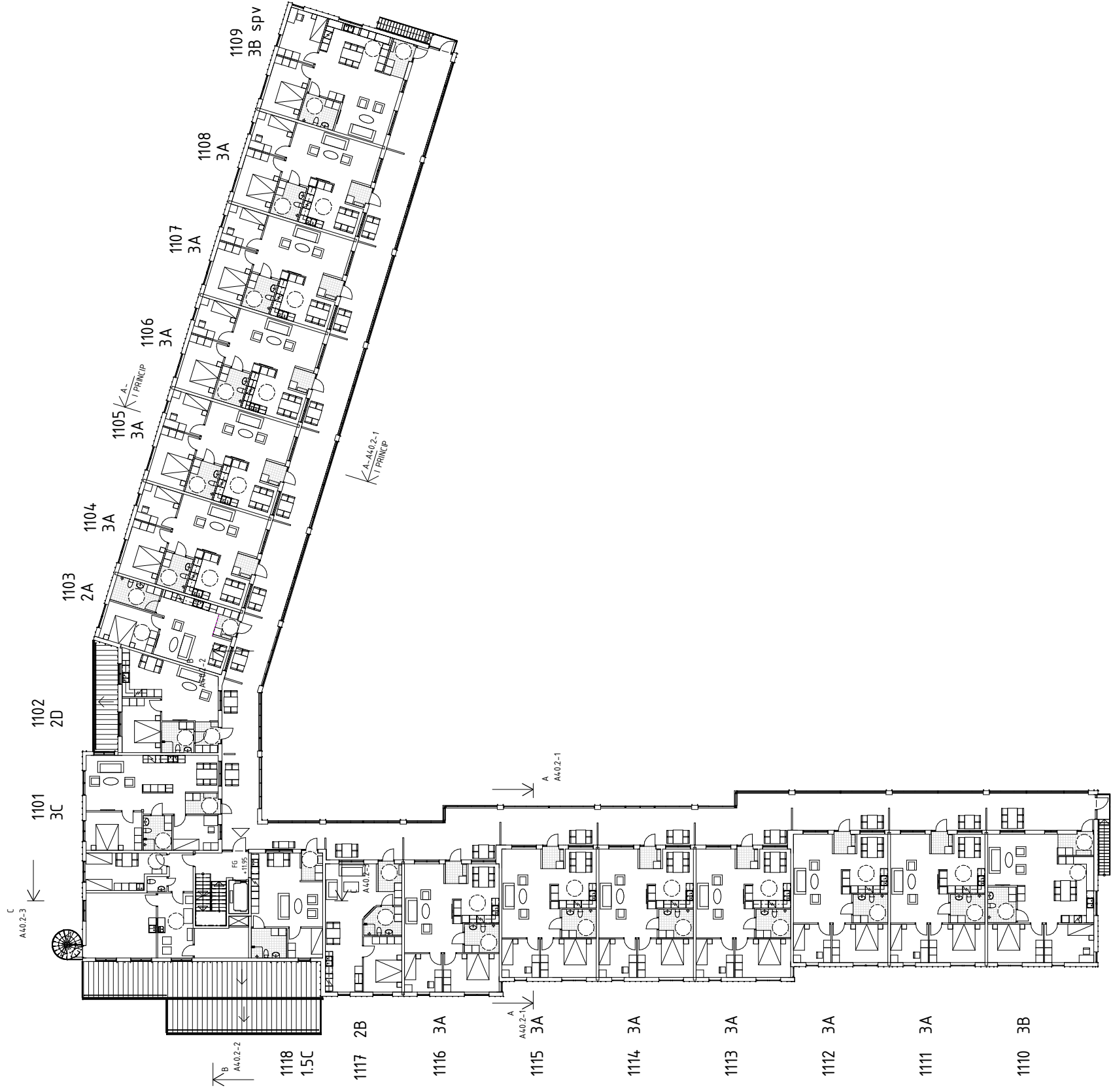
PLAN 2 1:200 (A3 1:400)
